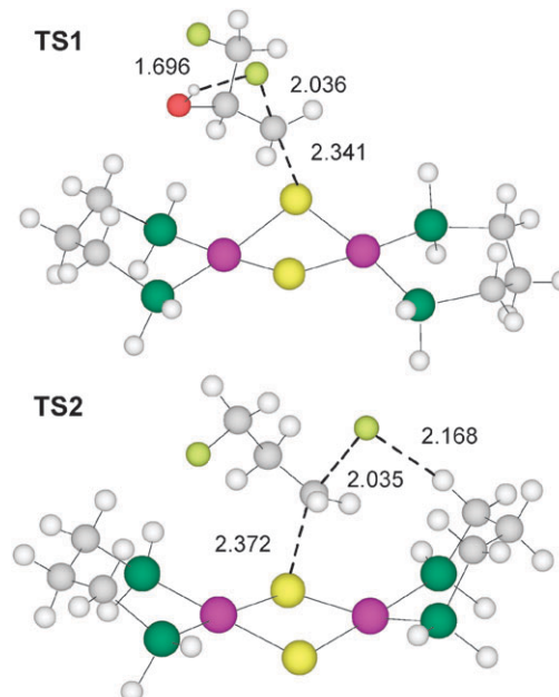
Fig. 2 Geometries of the transition states for the reaction of 2 with 1 ( TS1 ) or 4 ( TS2 ). Distances in Å. TS2 geometry obtained from ref. 19.
